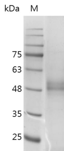
SDS-PAGE analysis of recombinant human HMGB1 C23AC45A
